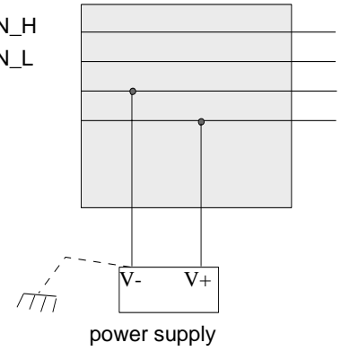
Flat media wiring terminal block open-style connector*
