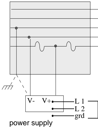
Round media wiring terminal
