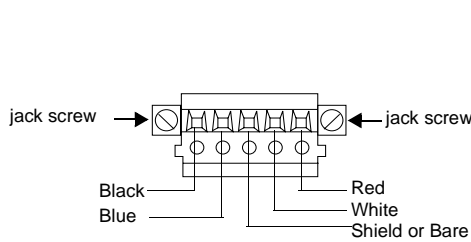
5-pin linear plug (open)
