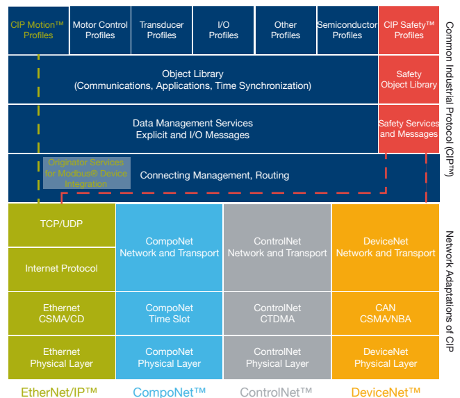
Figure 1: DeviceNet as Part of the CIP OSI Model
