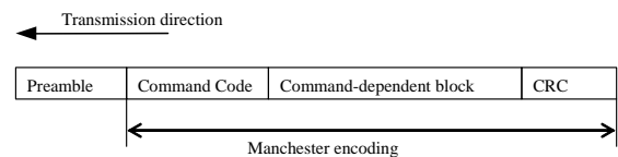
Figure 3 Frame block
