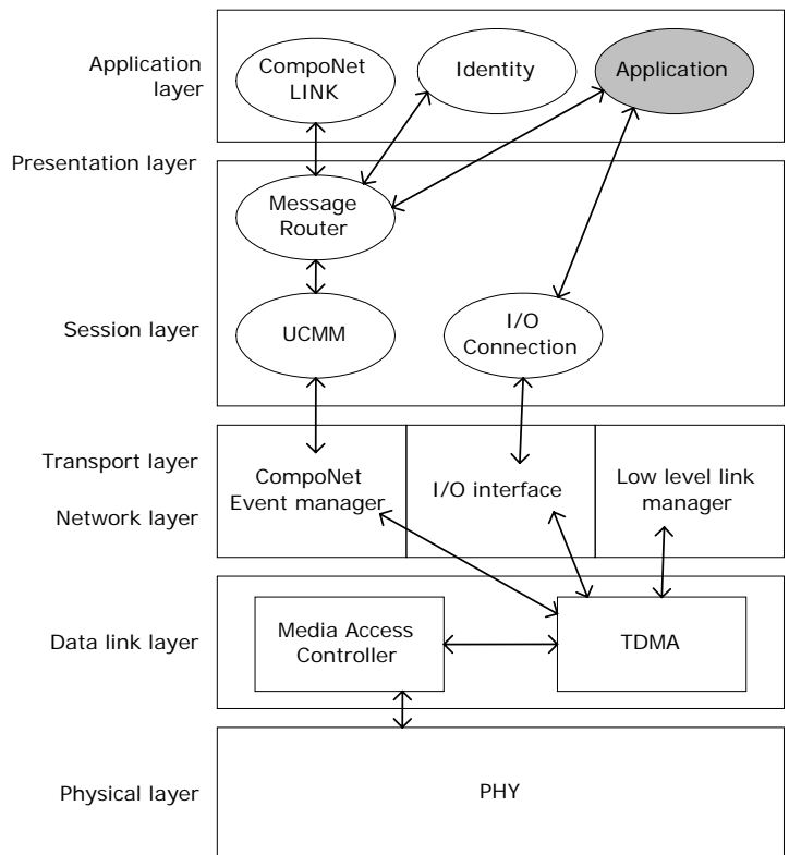
Figure 4 OSI Layer details
