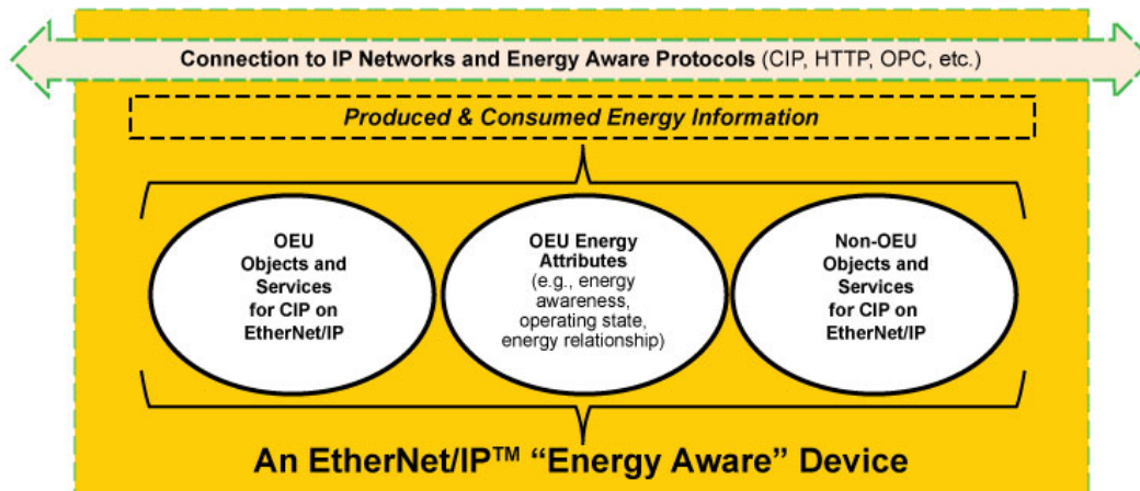
FIGURE 3: INFORMATION AND COMMUNICATION MODEL OF AN OEU-ENABLED ASSET
