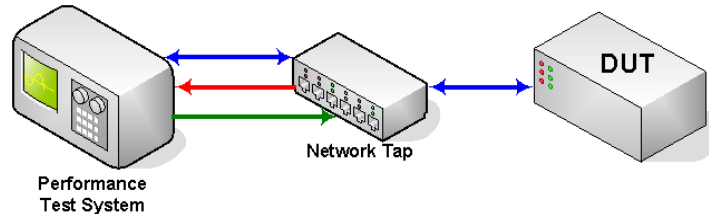
Figure 1 – Performance Test System Setup
