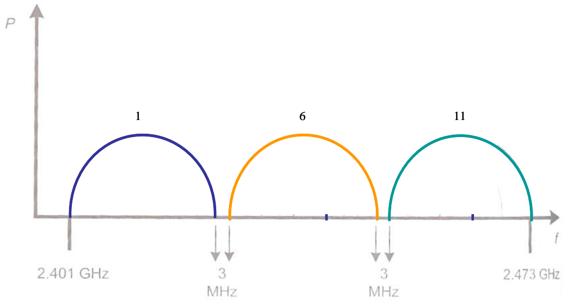
Figure 5. Non-overlapping 802.11bg Channels (1, 6 & 11)
