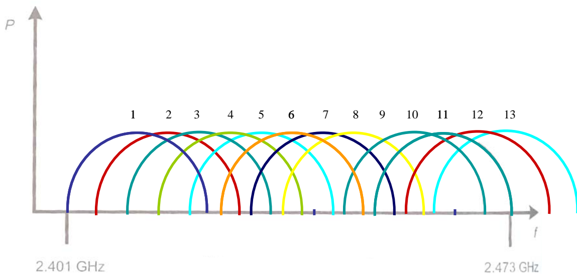
Figure 4. 802.11b/g Channels
