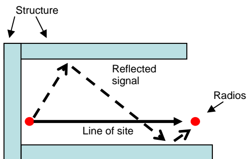
Figure 8. Multipath Phenomena
