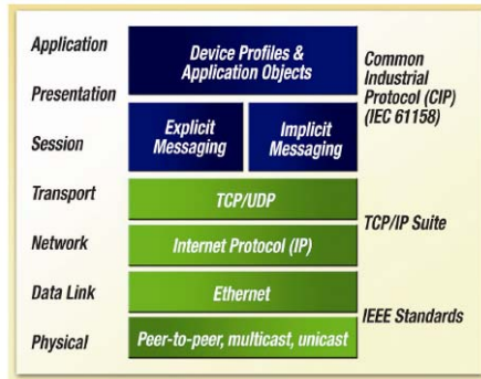
Figure 1: EtherNet/IP Protocol Stack
