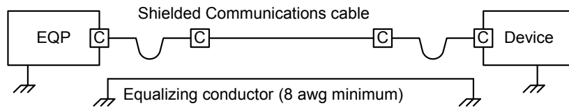
Figure 6 : Ground offset Equalizing Conductor (Equipotential)
