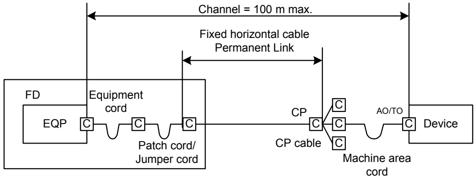
Figure 4 : Cross Connect AO/TO with CP Model
